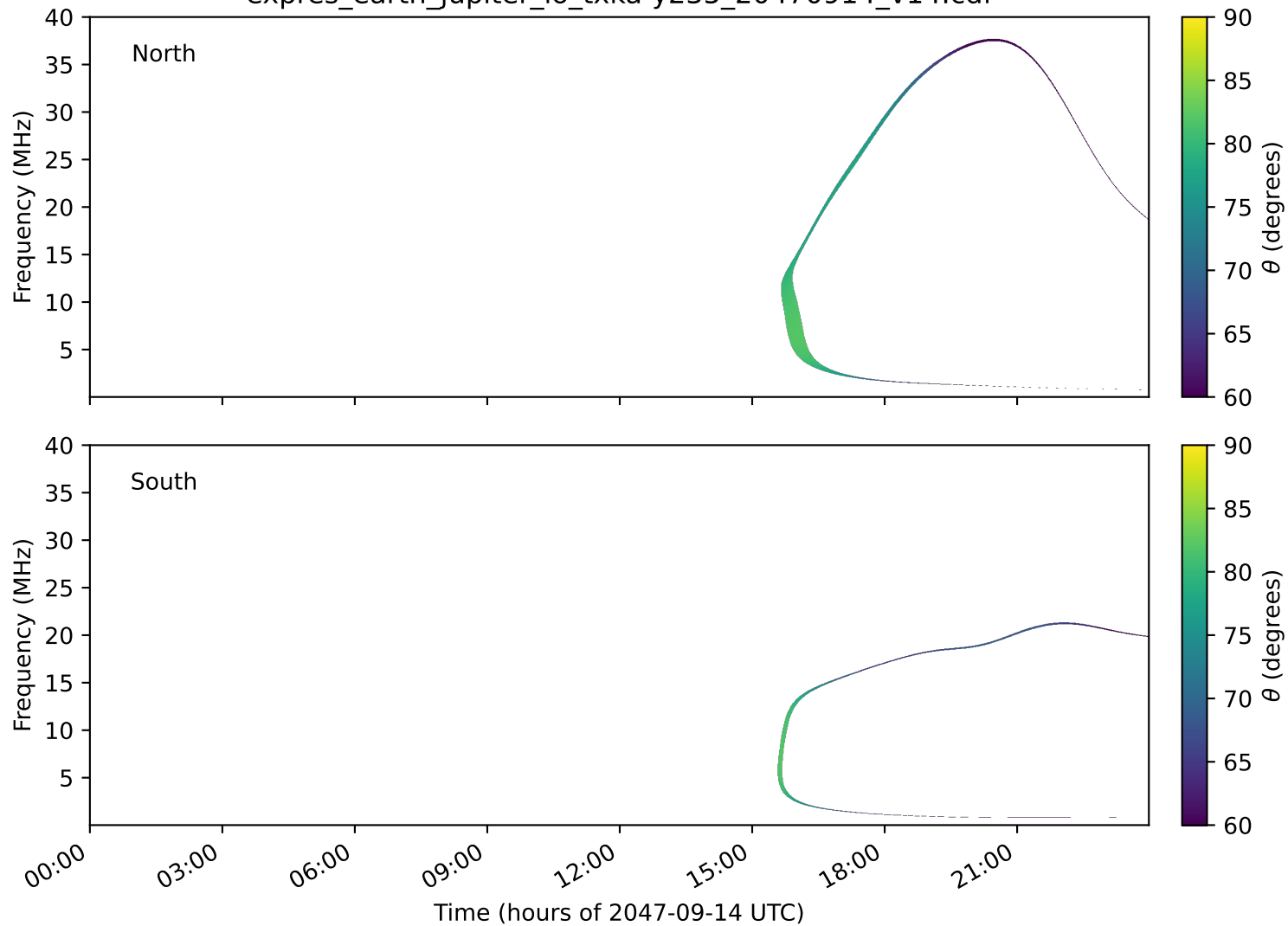
expres_earth_jupiter_io_txka-y235_20470914_v14.cdf
