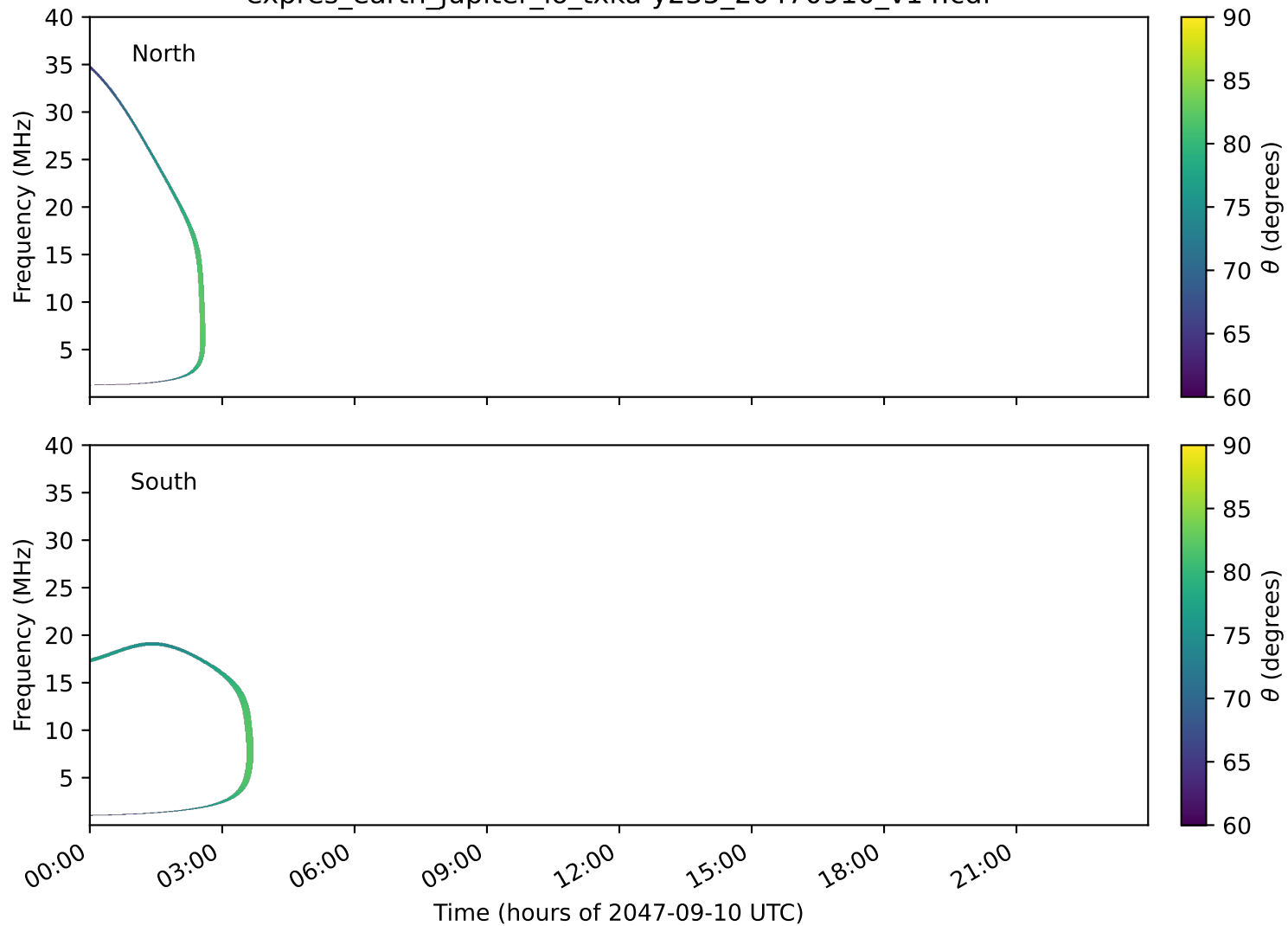
expres_earth_jupiter_io_txka-y235_20470910_v14.cdf
