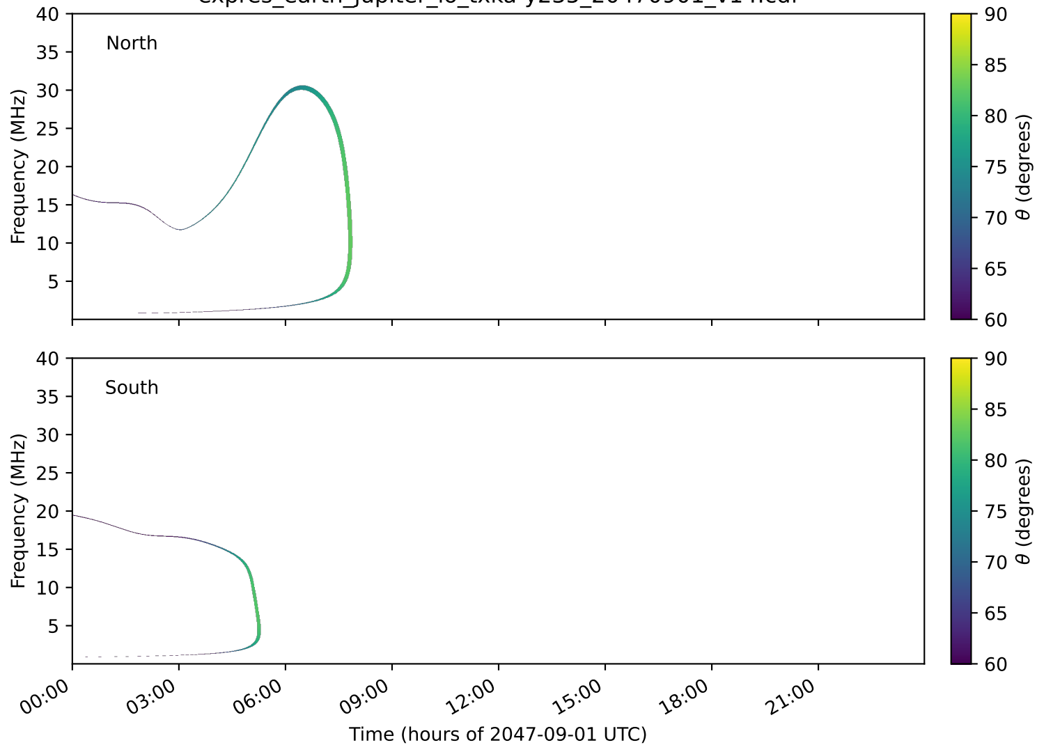
expres_earth_jupiter_io_txka-y235_20470901_v14.cdf
