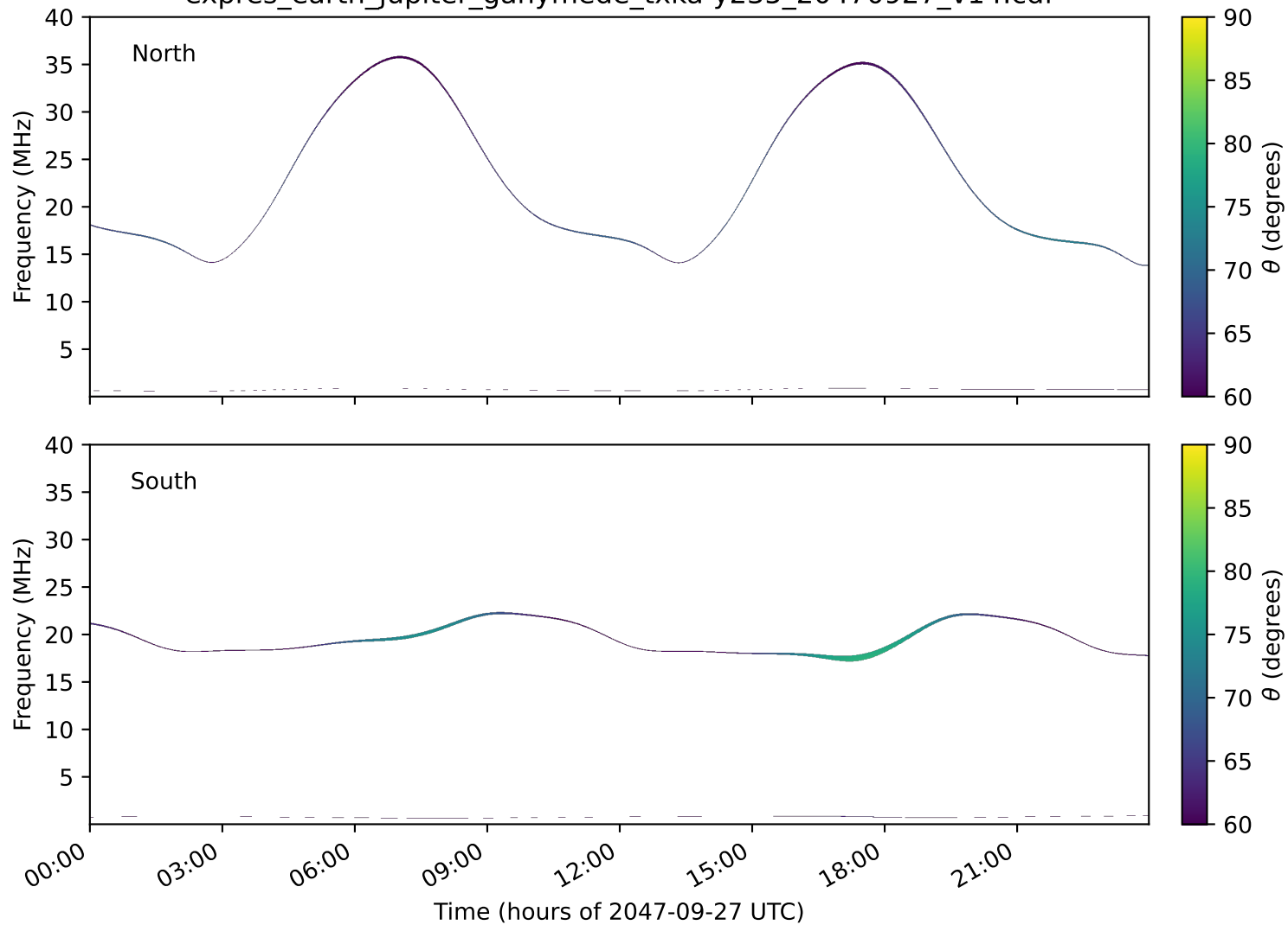
expres_earth_jupiter_ganymede_txka-y235_20470927_v14.cdf
