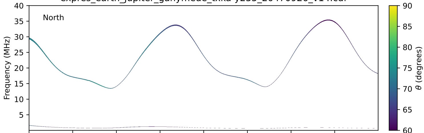
expres_earth_jupiter_ganymede_txka-y235_20470926_v14.cdf
