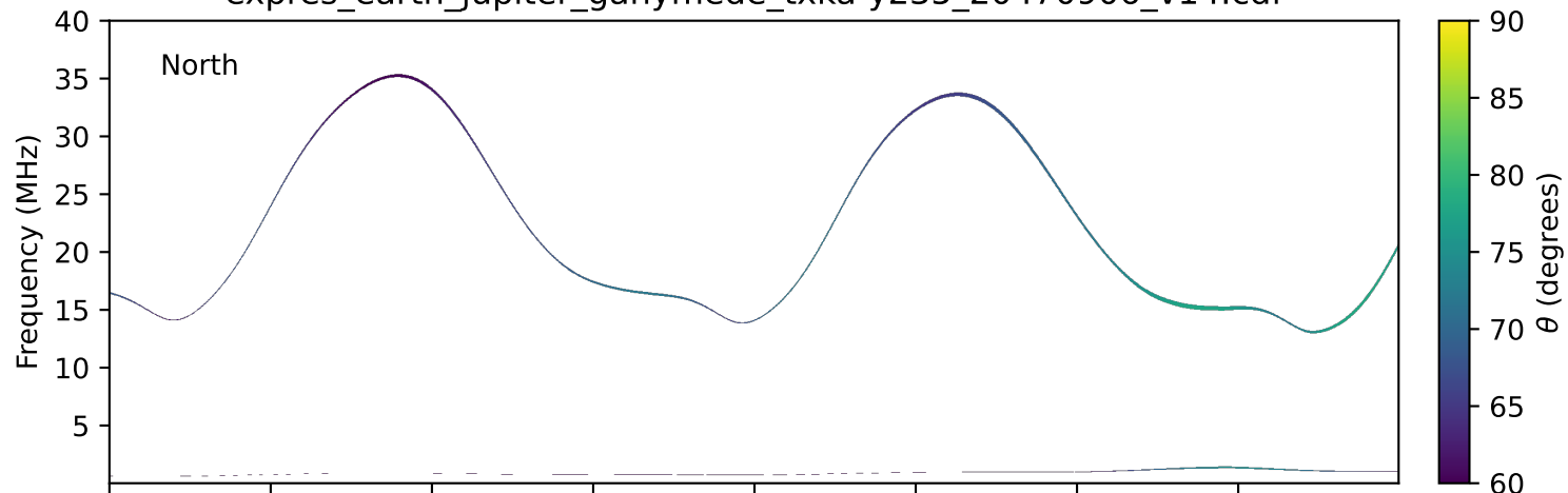
expres_earth_jupiter_ganymede_txka-y235_20470906_v14.cdf
