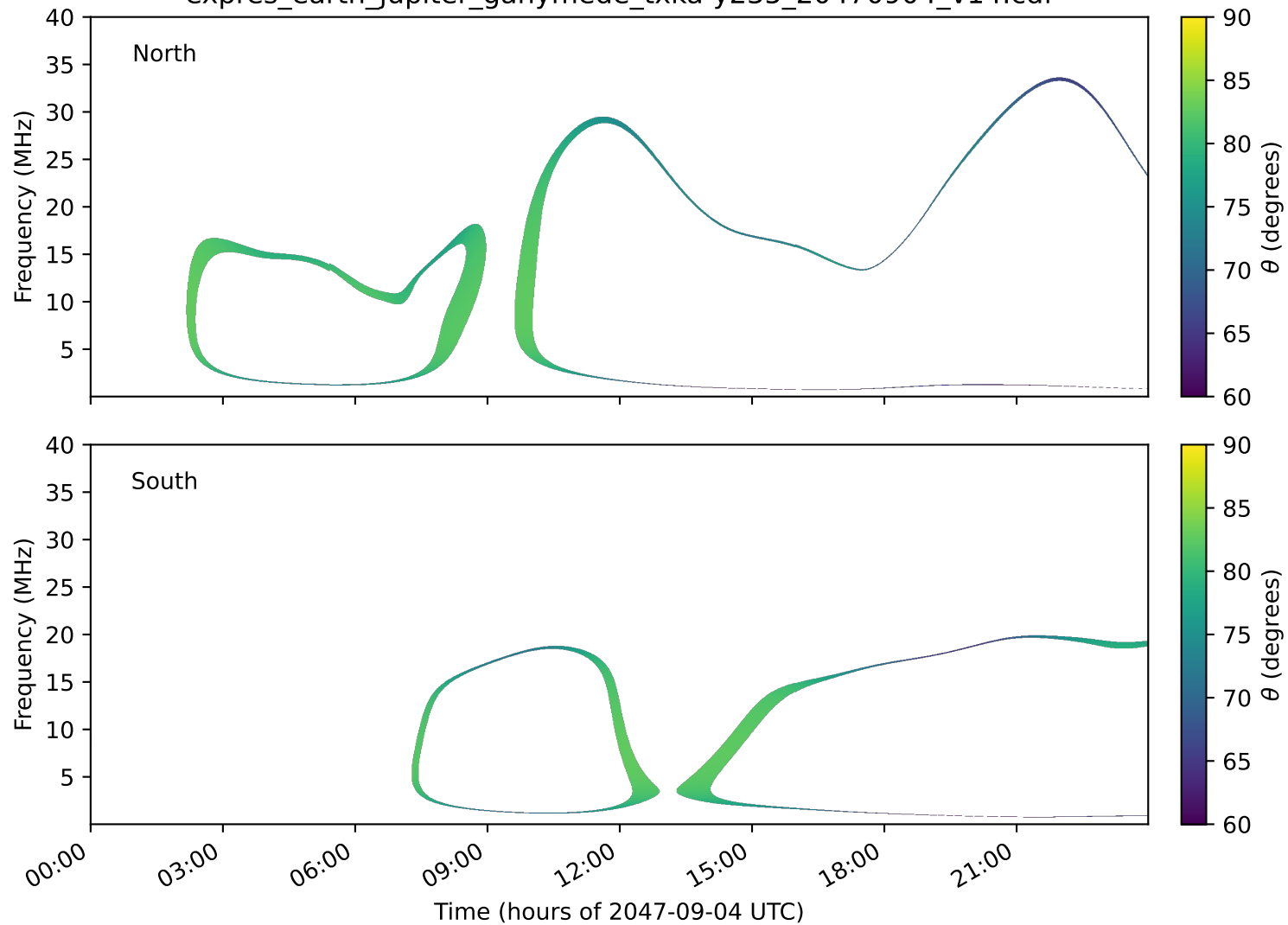
expres_earth_jupiter_ganymede_txka-y235_20470904_v14.cdf
