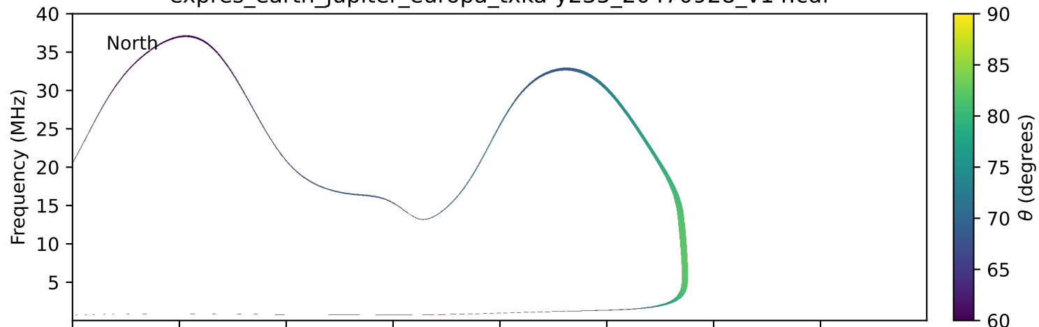
expres_earth_jupiter_europa_txka-y235_20470928_v14.cdf
