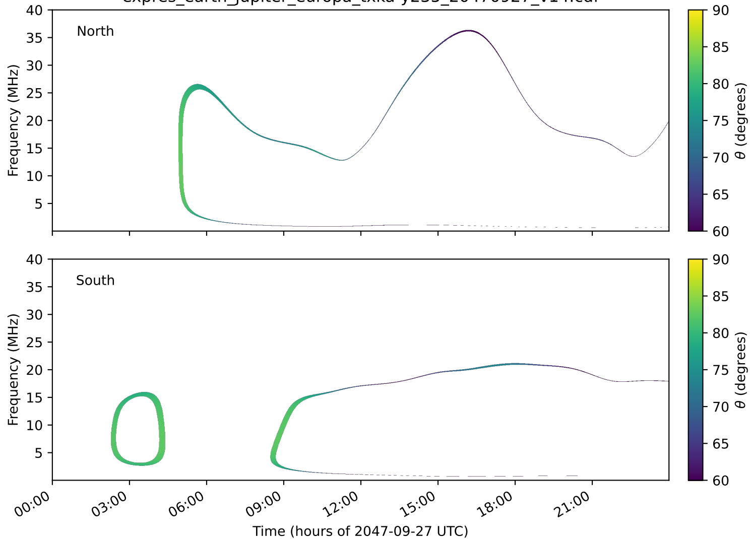
expres_earth_jupiter_europa_txka-y235_20470927_v14.cdf
