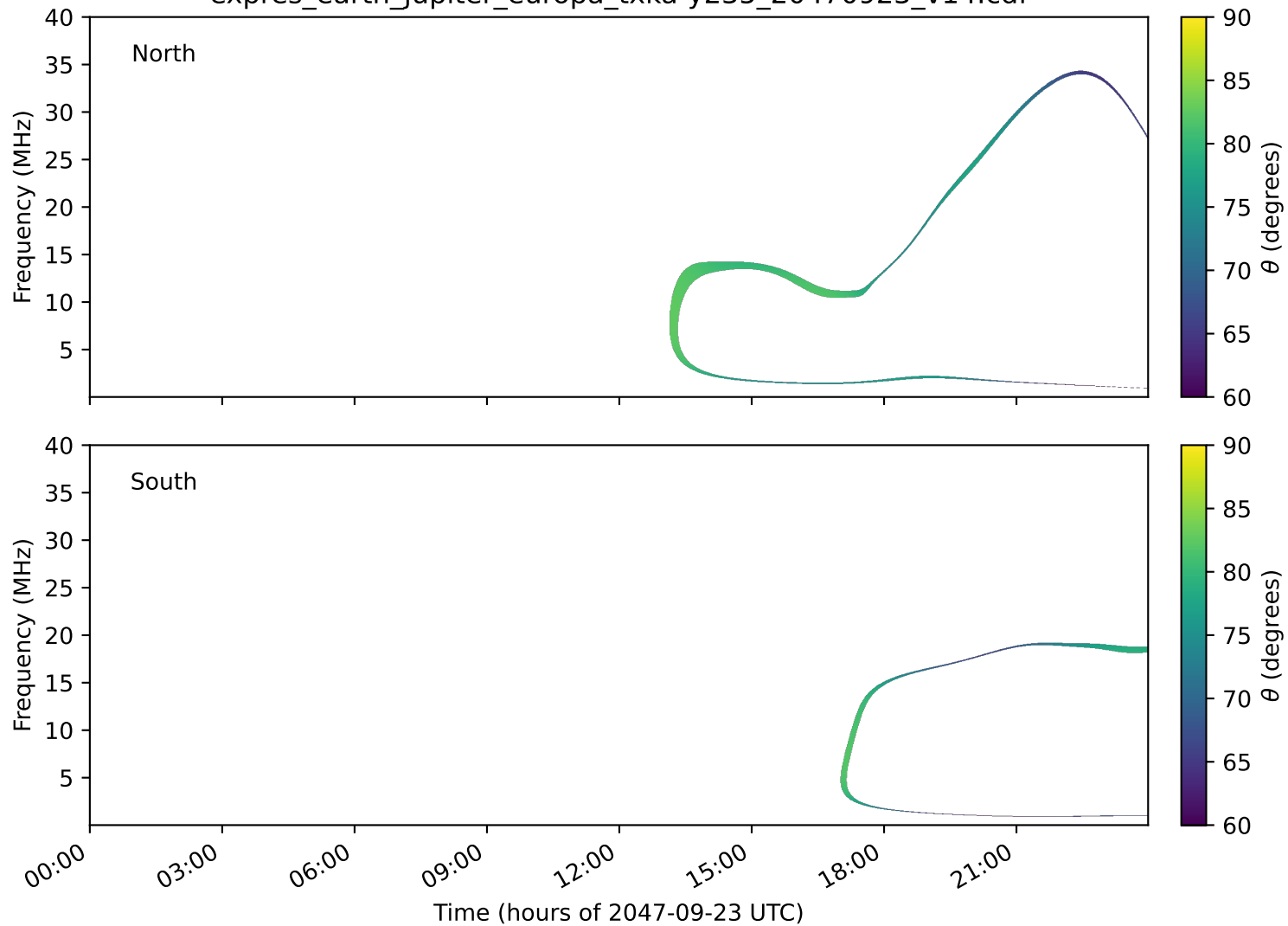
expres_earth_jupiter_europa_txka-y235_20470923_v14.cdf
