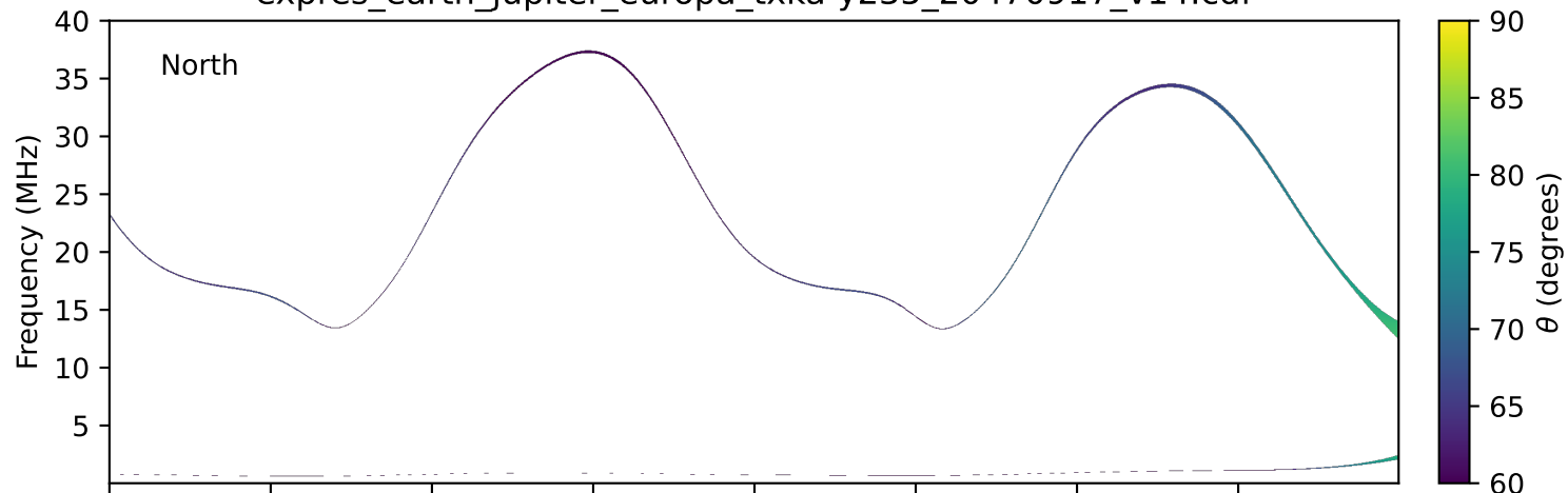
expres_earth_jupiter_europa_txka-y235_20470917_v14.cdf
