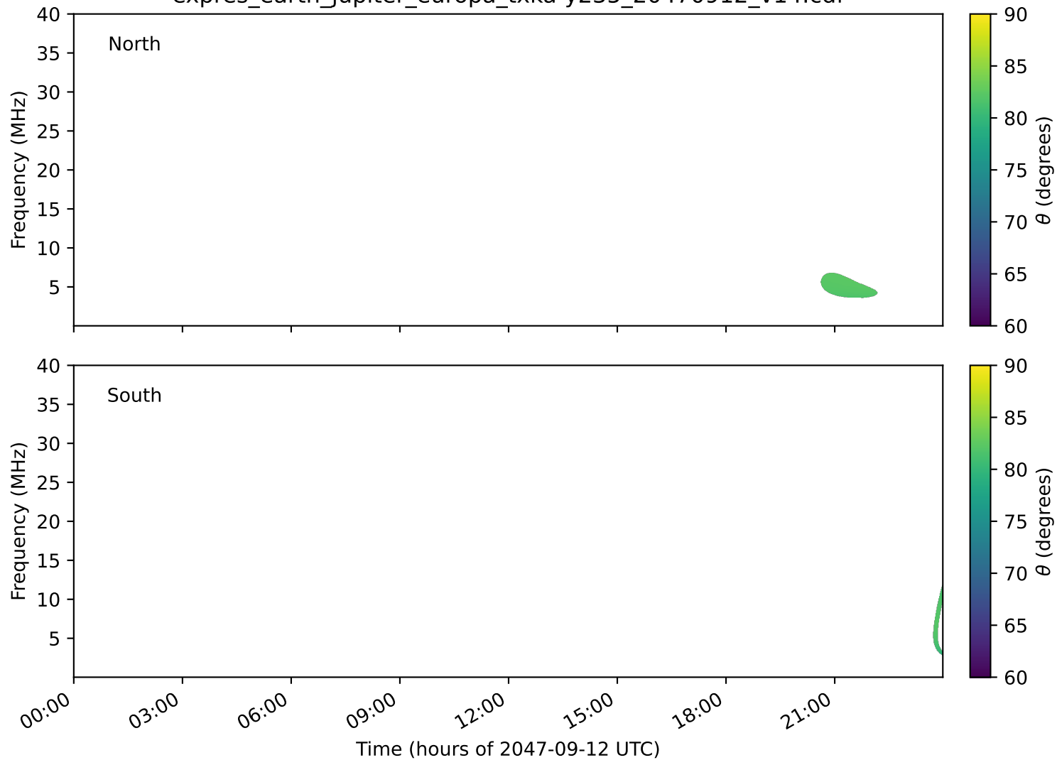
expres_earth_jupiter_europa_txka-y235_20470912_v14.cdf
