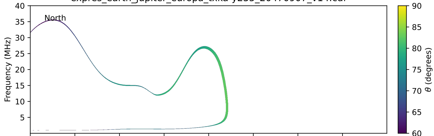
expres_earth_jupiter_europa_txka-y235_20470907_v14.cdf
