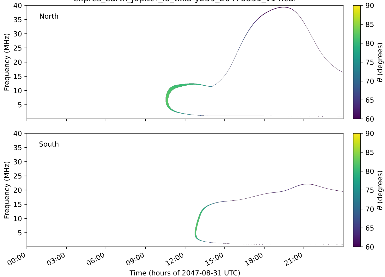
expres_earth_jupiter_io_txka-y235_20470831_v14.cdf
