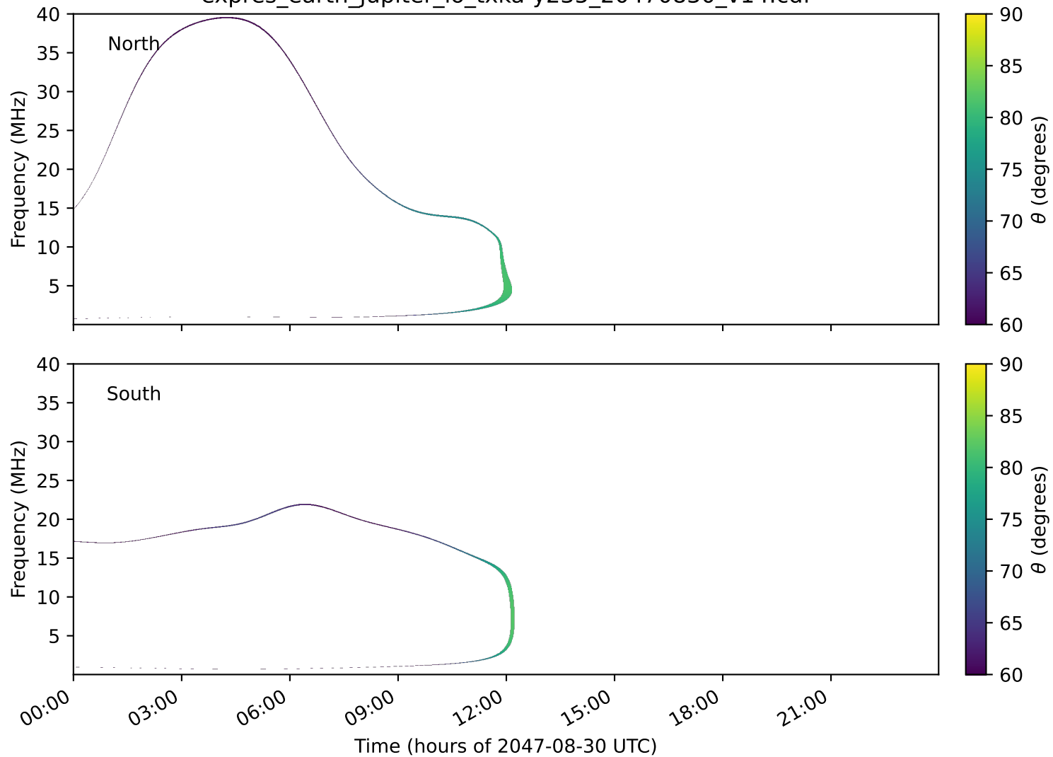
expres_earth_jupiter_io_txka-y235_20470830_v14.cdf
