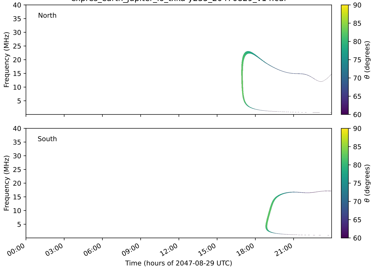
expres_earth_jupiter_io_txka-y235_20470829_v14.cdf
