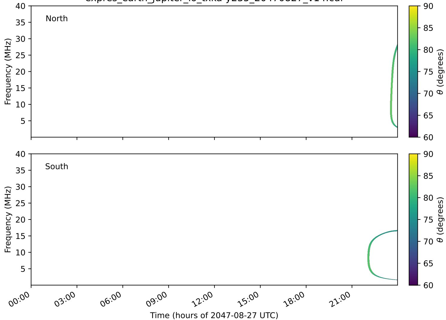
expres_earth_jupiter_io_txka-y235_20470827_v14.cdf
