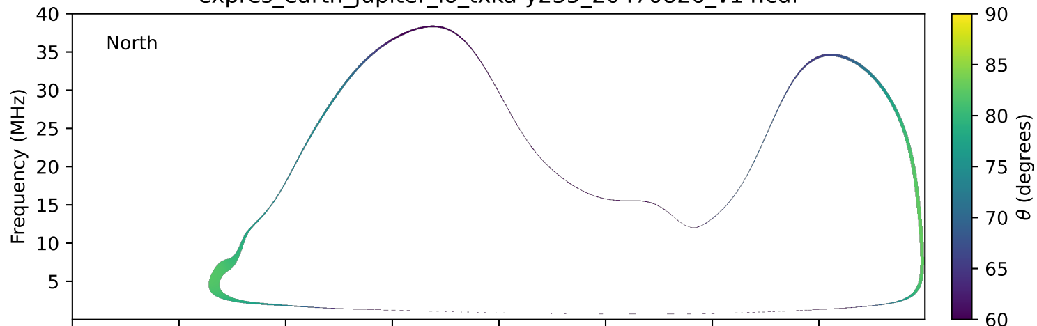
expres_earth_jupiter_io_txka-y235_20470826_v14.cdf
