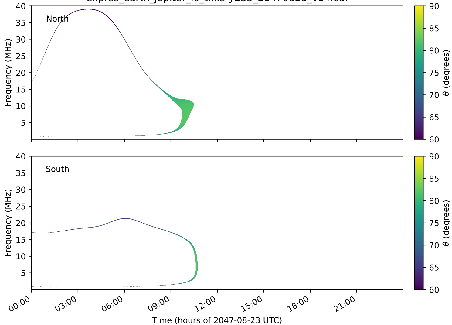
expres_earth_jupiter_io_txka-y235_20470823_v14.cdf
