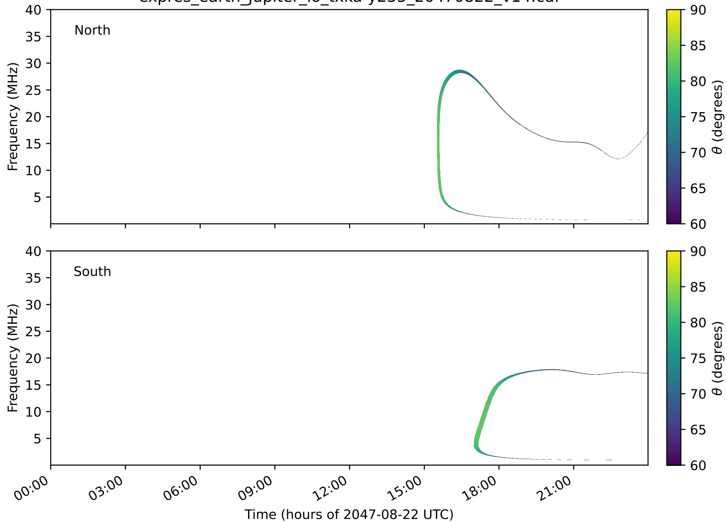
expres_earth_jupiter_io_txka-y235_20470822_v14.cdf
