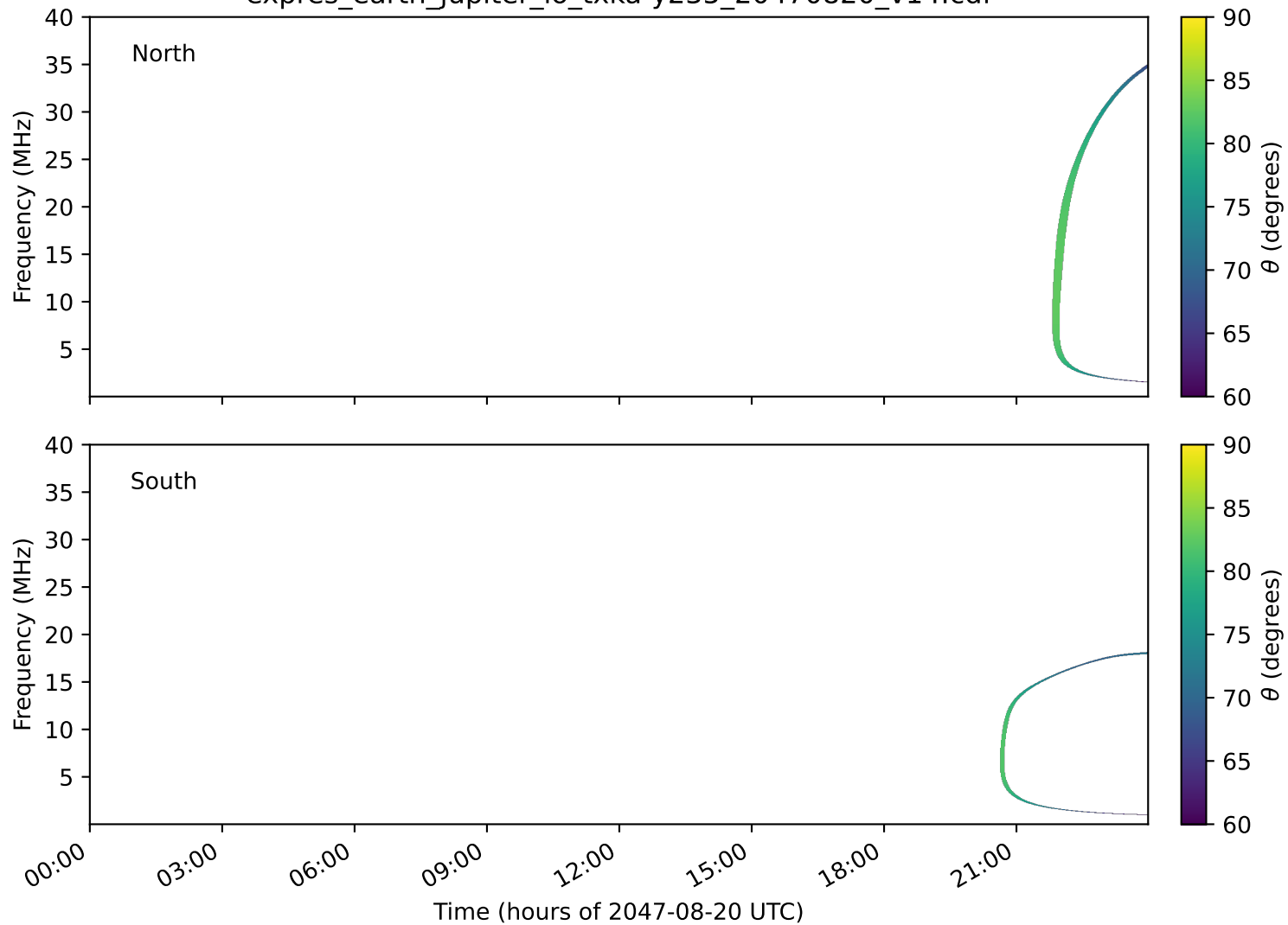
expres_earth_jupiter_io_txka-y235_20470820_v14.cdf
