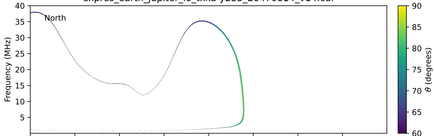
expres_earth_jupiter_io_txka-y235_20470814_v14.cdf
