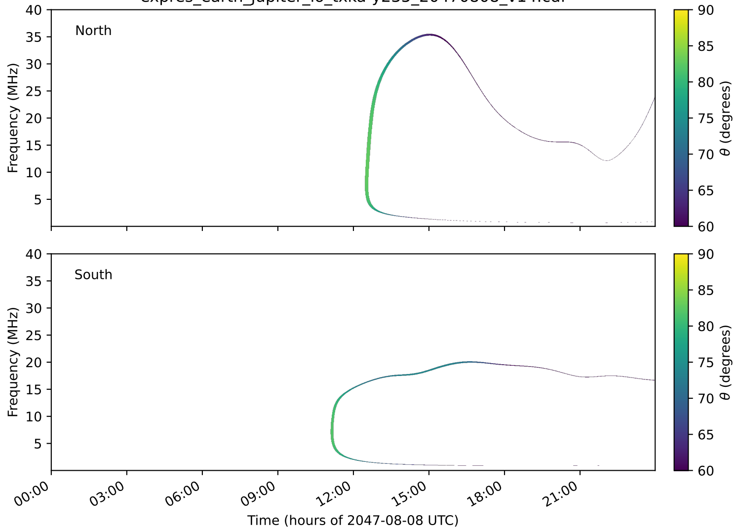
expres_earth_jupiter_io_txka-y235_20470808_v14.cdf
