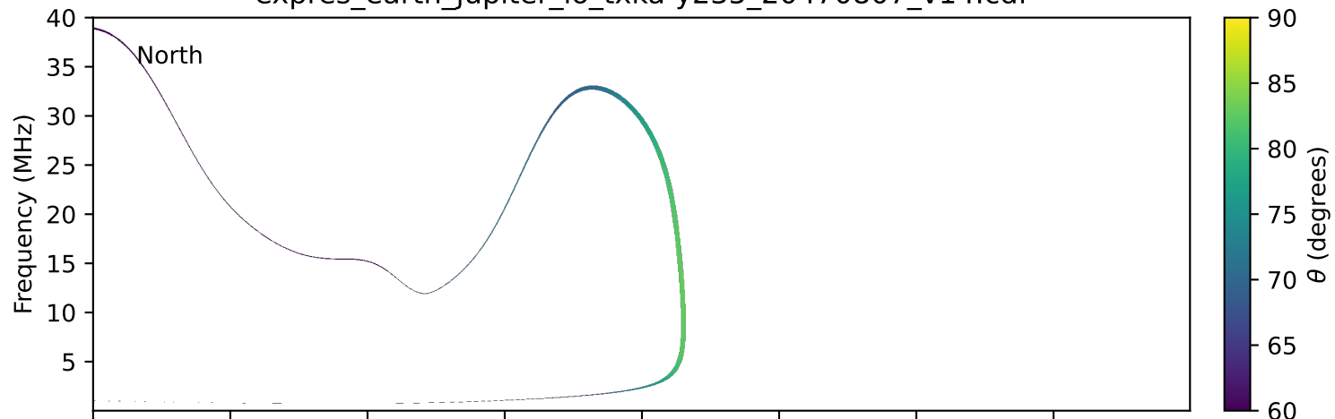
expres_earth_jupiter_io_txka-y235_20470807_v14.cdf
