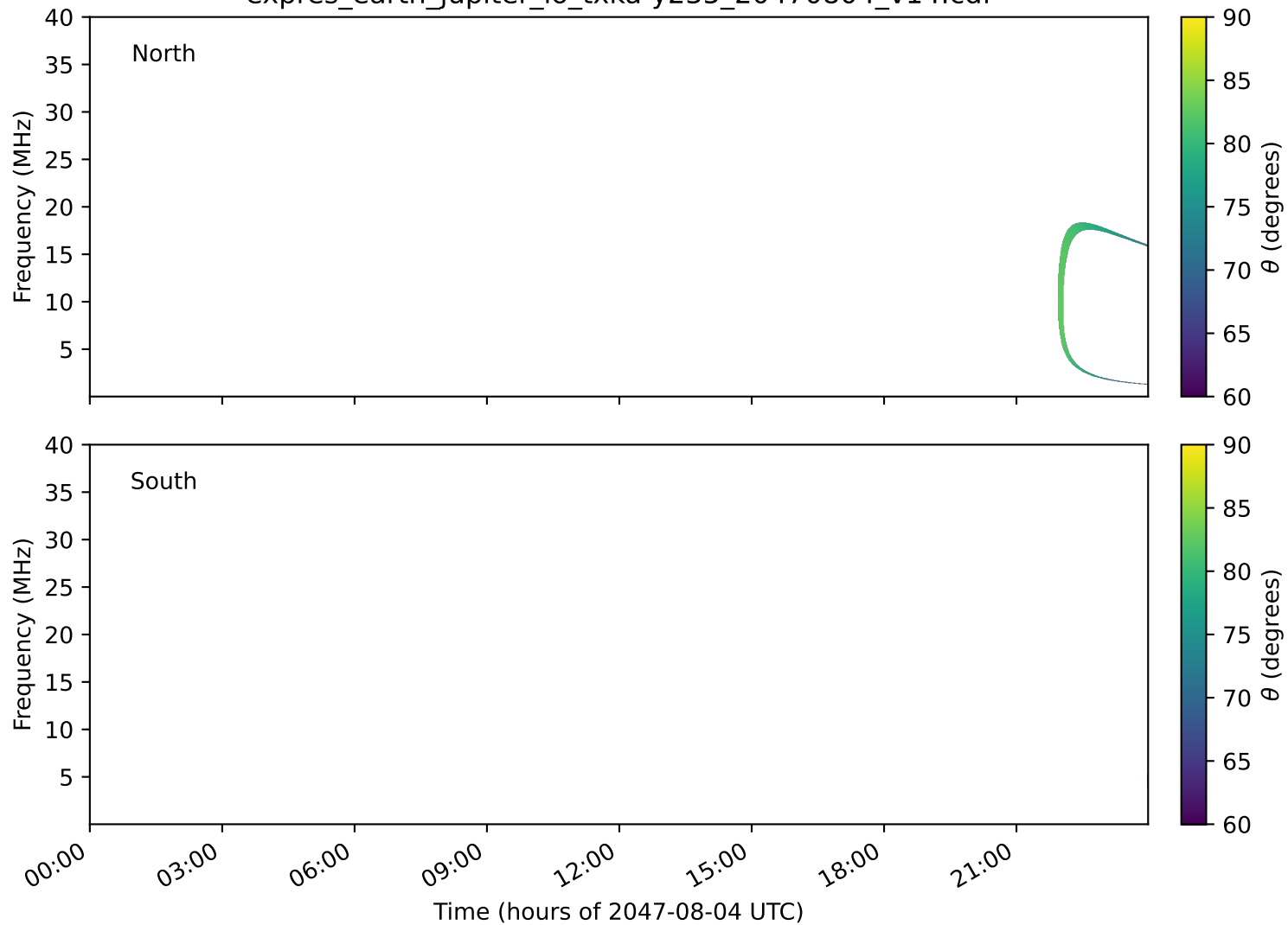
expres_earth_jupiter_io_txka-y235_20470804_v14.cdf
