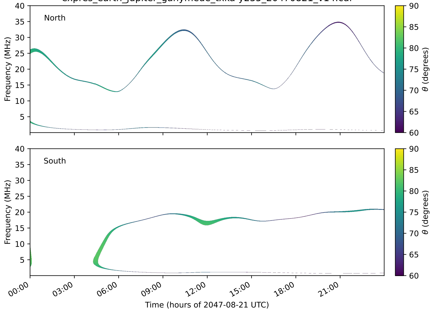
expres_earth_jupiter_ganymede_txka-y235_20470821_v14.cdf
