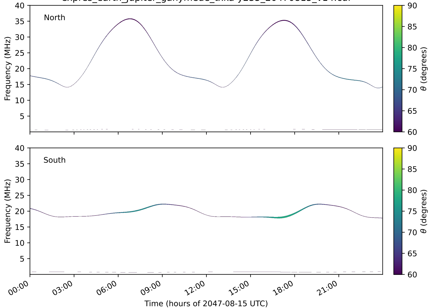
expres_earth_jupiter_ganymede_txka-y235_20470815_v14.cdf
