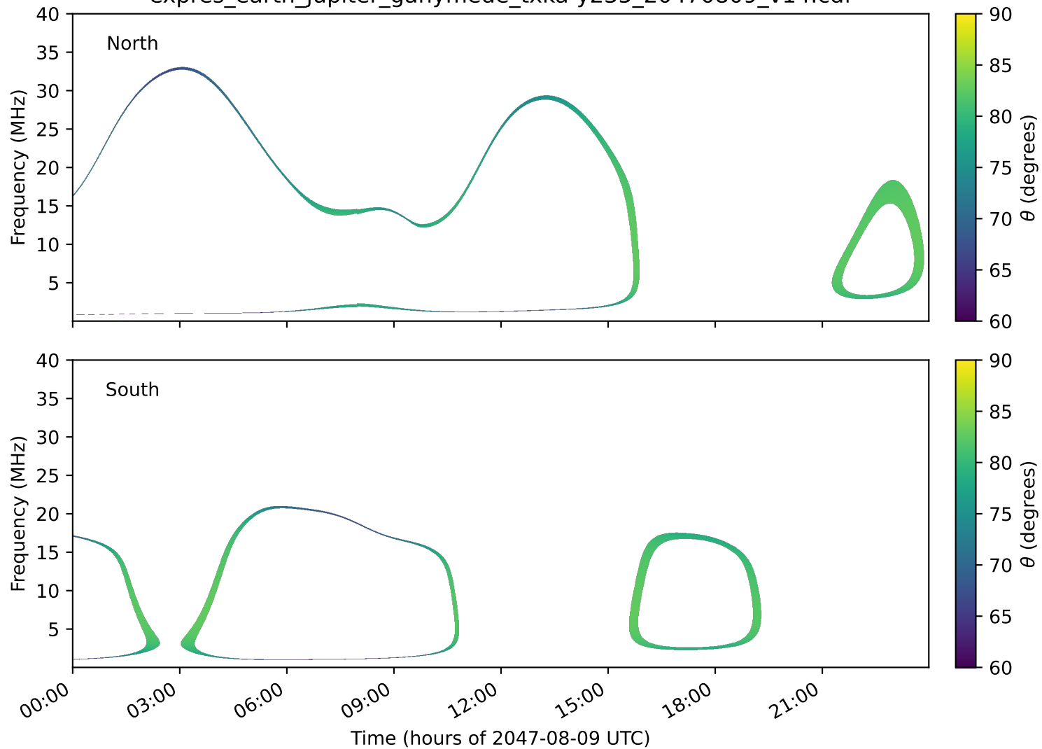
expres_earth_jupiter_ganymede_txka-y235_20470809_v14.cdf
