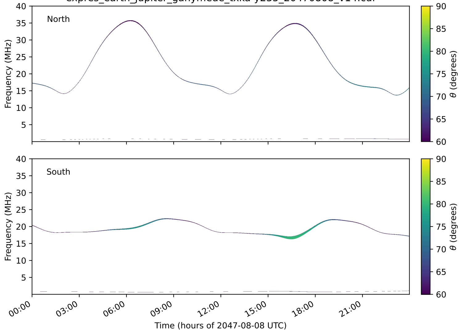
expres_earth_jupiter_ganymede_txka-y235_20470808_v14.cdf
