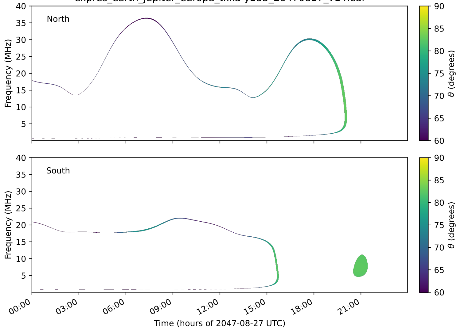
expres_earth_jupiter_europa_txka-y235_20470827_v14.cdf
