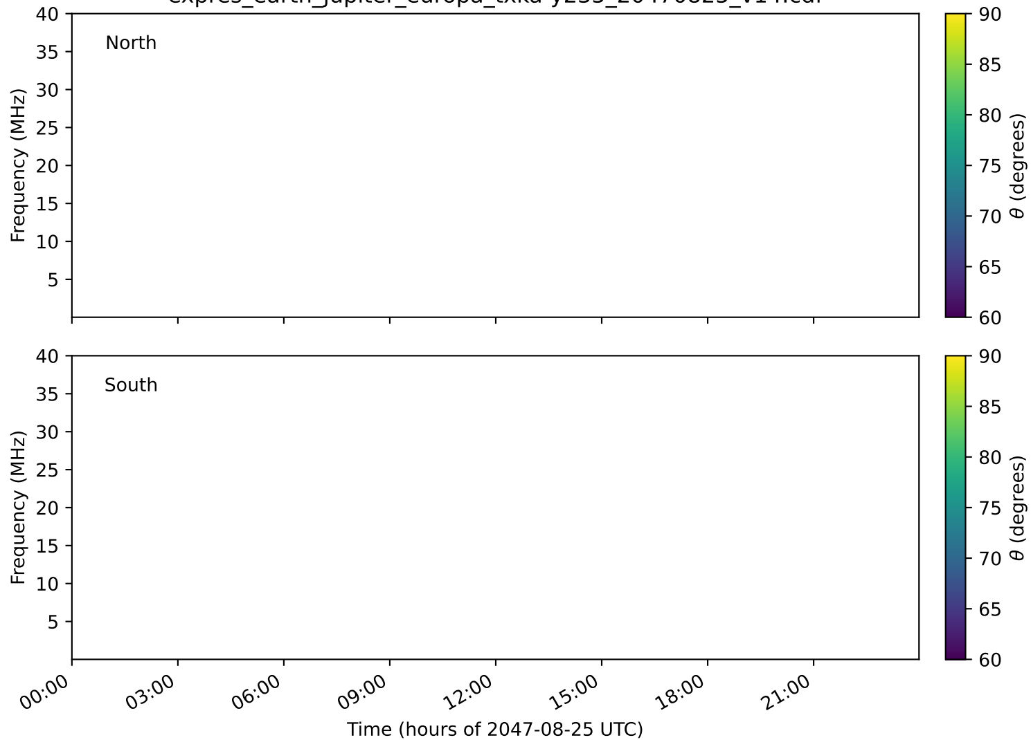
expres_earth_jupiter_europa_txka-y235_20470825_v14.cdf
