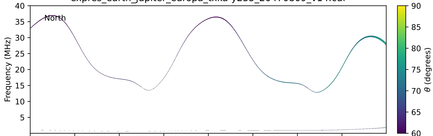
expres_earth_jupiter_europa_txka-y235_20470809_v14.cdf
