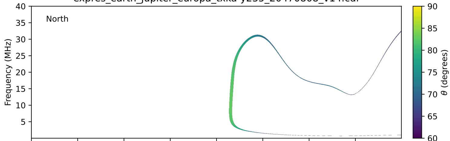
expres_earth_jupiter_europa_txka-y235_20470808_v14.cdf
