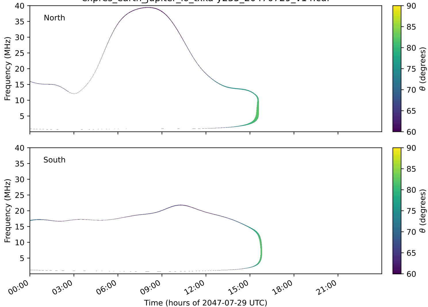
expres_earth_jupiter_io_txka-y235_20470729_v14.cdf
