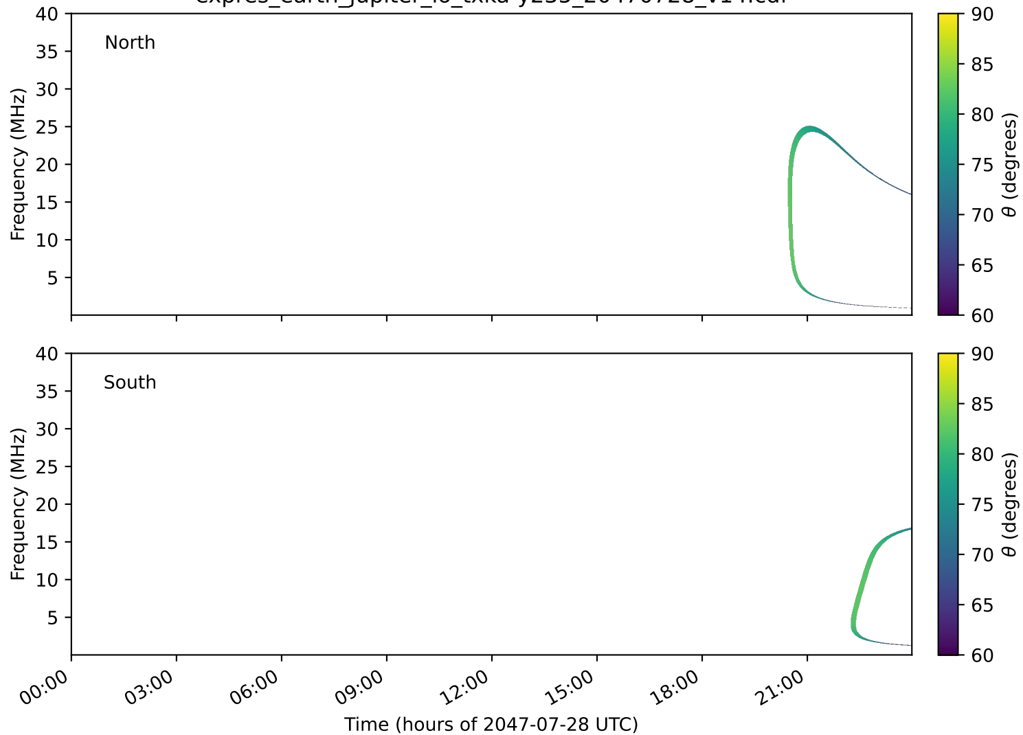
expres_earth_jupiter_io_txka-y235_20470728_v14.cdf
