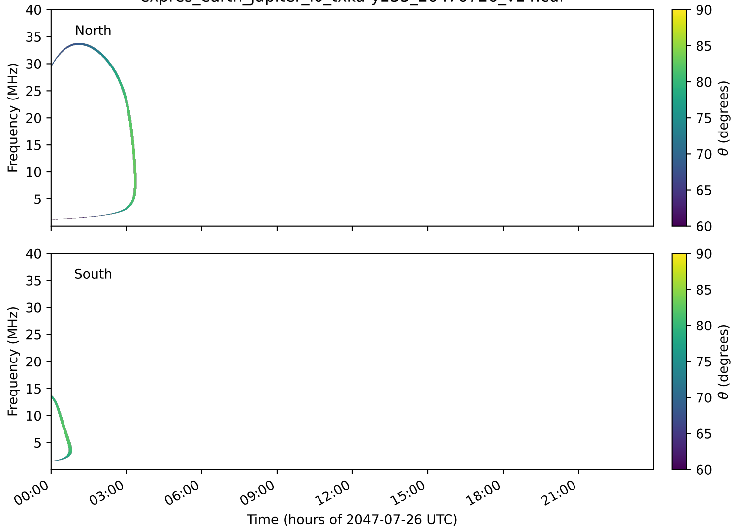
expres_earth_jupiter_io_txka-y235_20470726_v14.cdf
