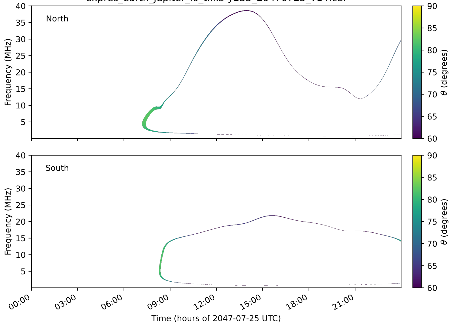
expres_earth_jupiter_io_txka-y235_20470725_v14.cdf
