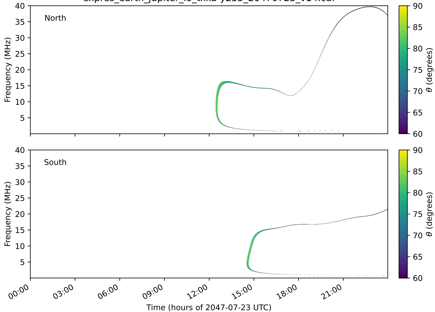
expres_earth_jupiter_io_txka-y235_20470723_v14.cdf
