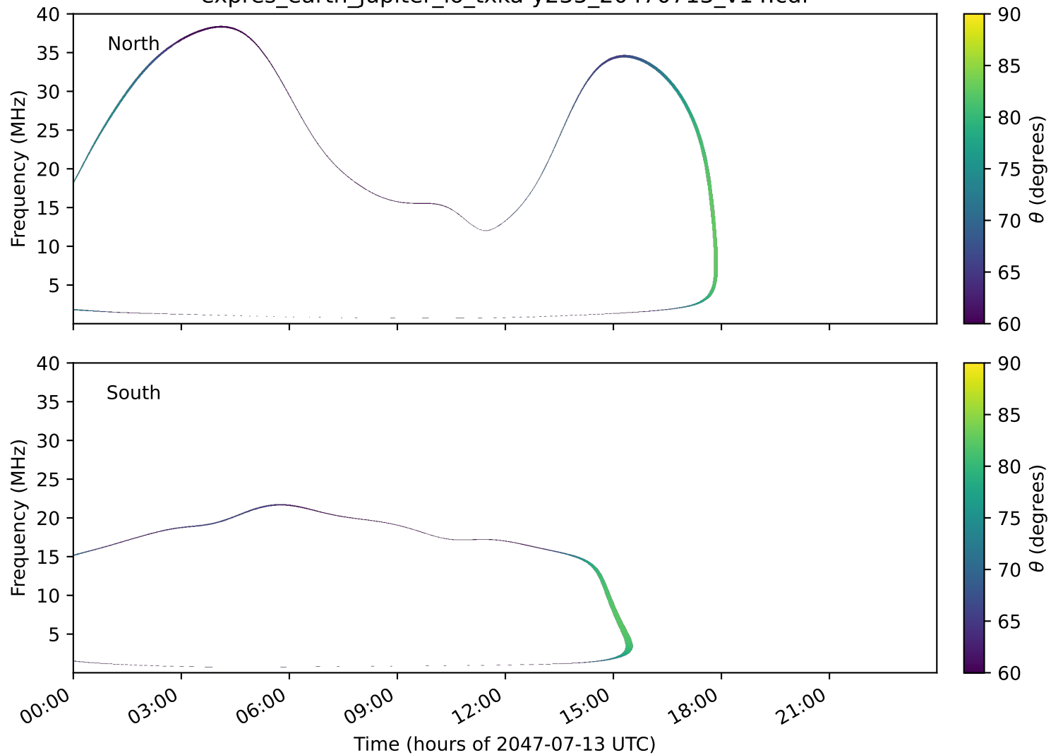
expres_earth_jupiter_io_txka-y235_20470713_v14.cdf
