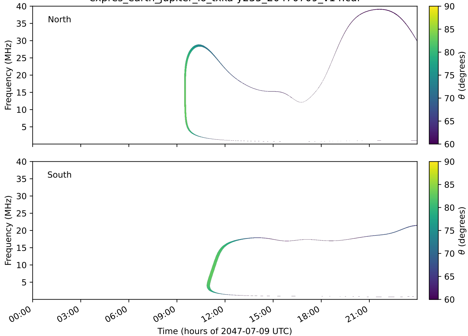
expres_earth_jupiter_io_txka-y235_20470709_v14.cdf
