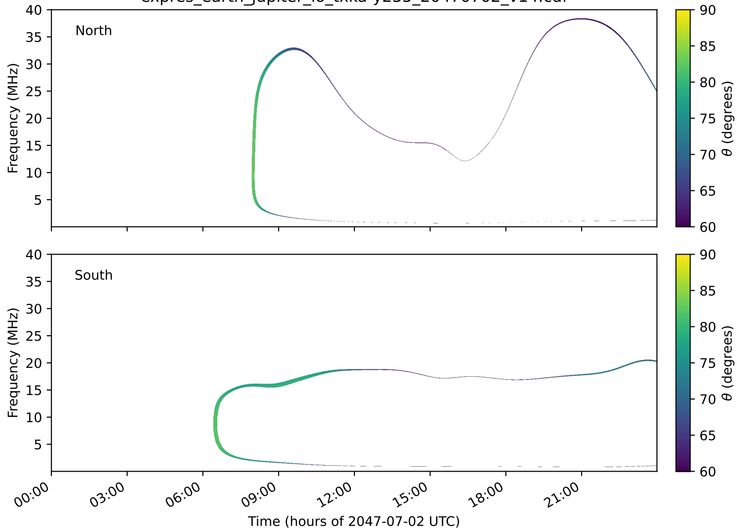
expres_earth_jupiter_io_txka-y235_20470702_v14.cdf
