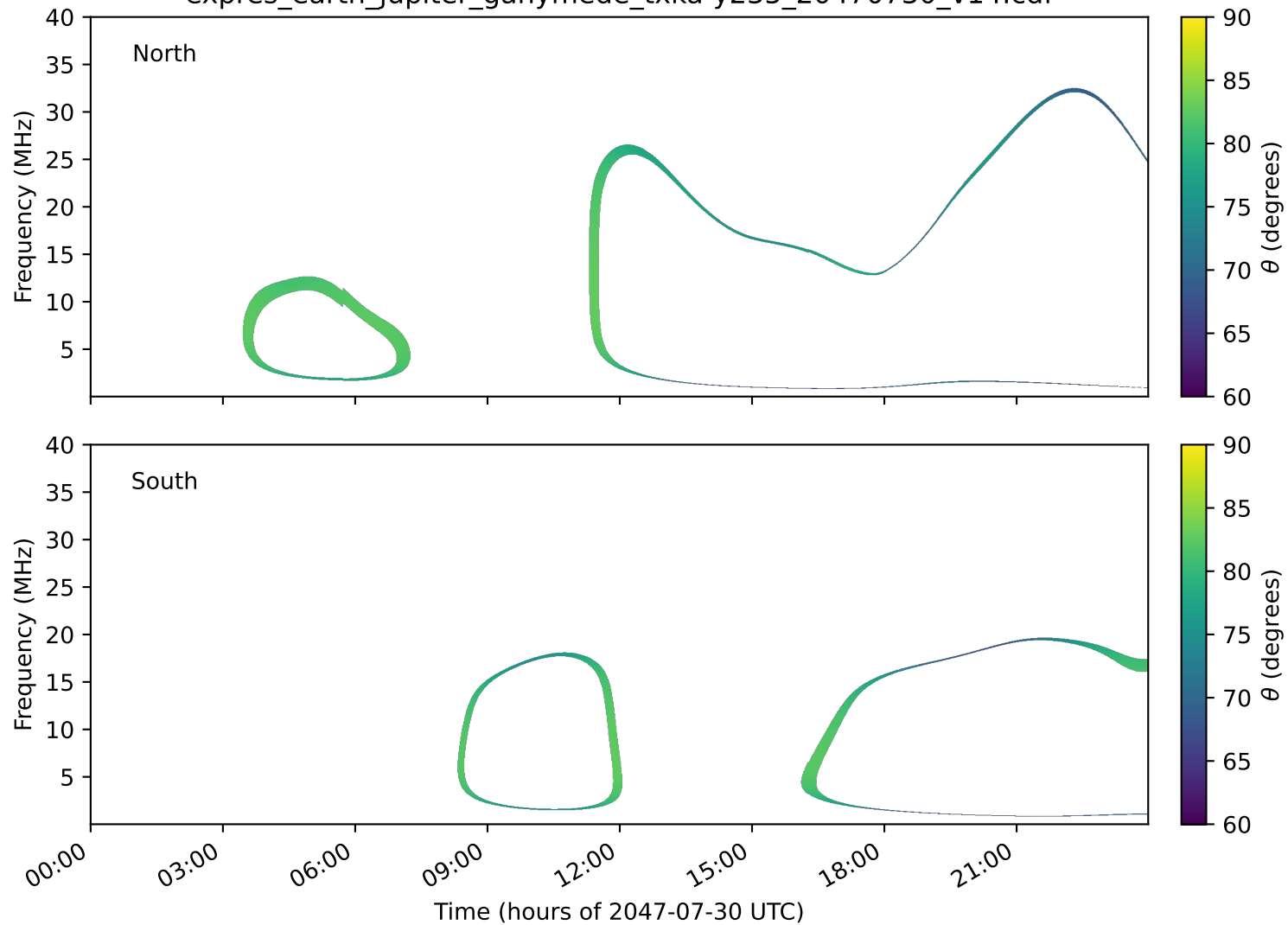
expres_earth_jupiter_ganymede_txka-y235_20470730_v14.cdf
