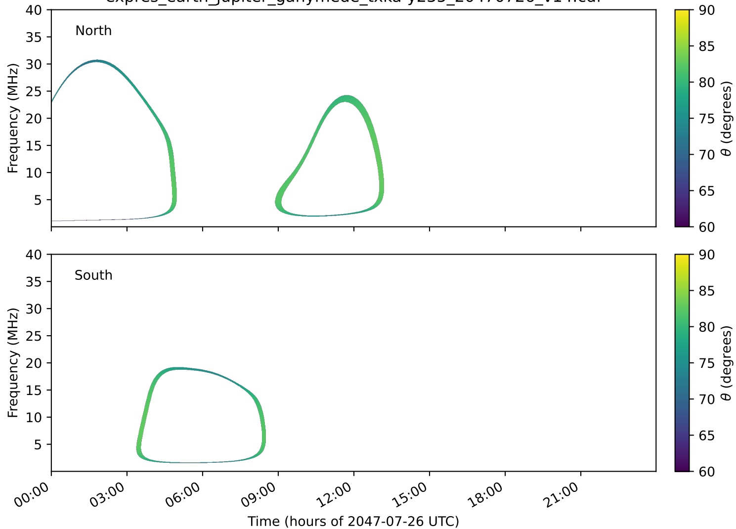
expres_earth_jupiter_ganymede_txka-y235_20470726_v14.cdf
