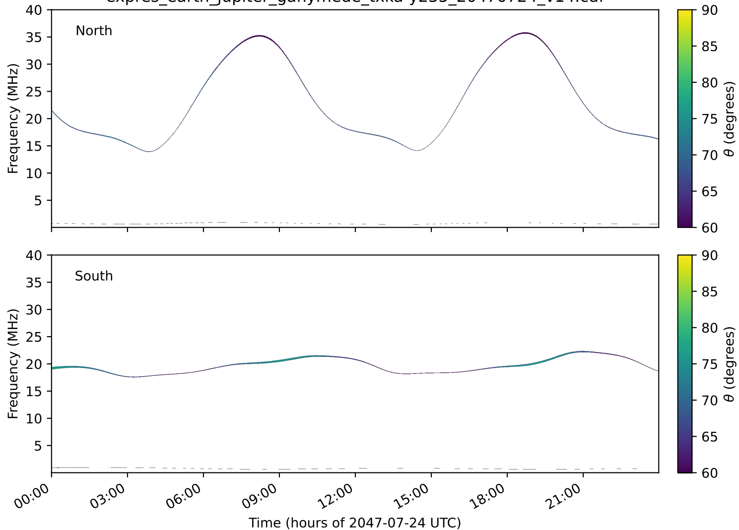
expres_earth_jupiter_ganymede_txka-y235_20470724_v14.cdf
