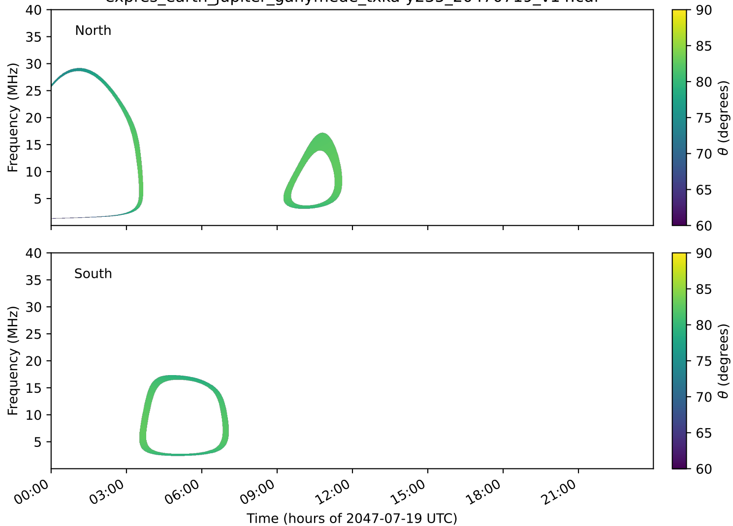
expres_earth_jupiter_ganymede_txka-y235_20470719_v14.cdf
