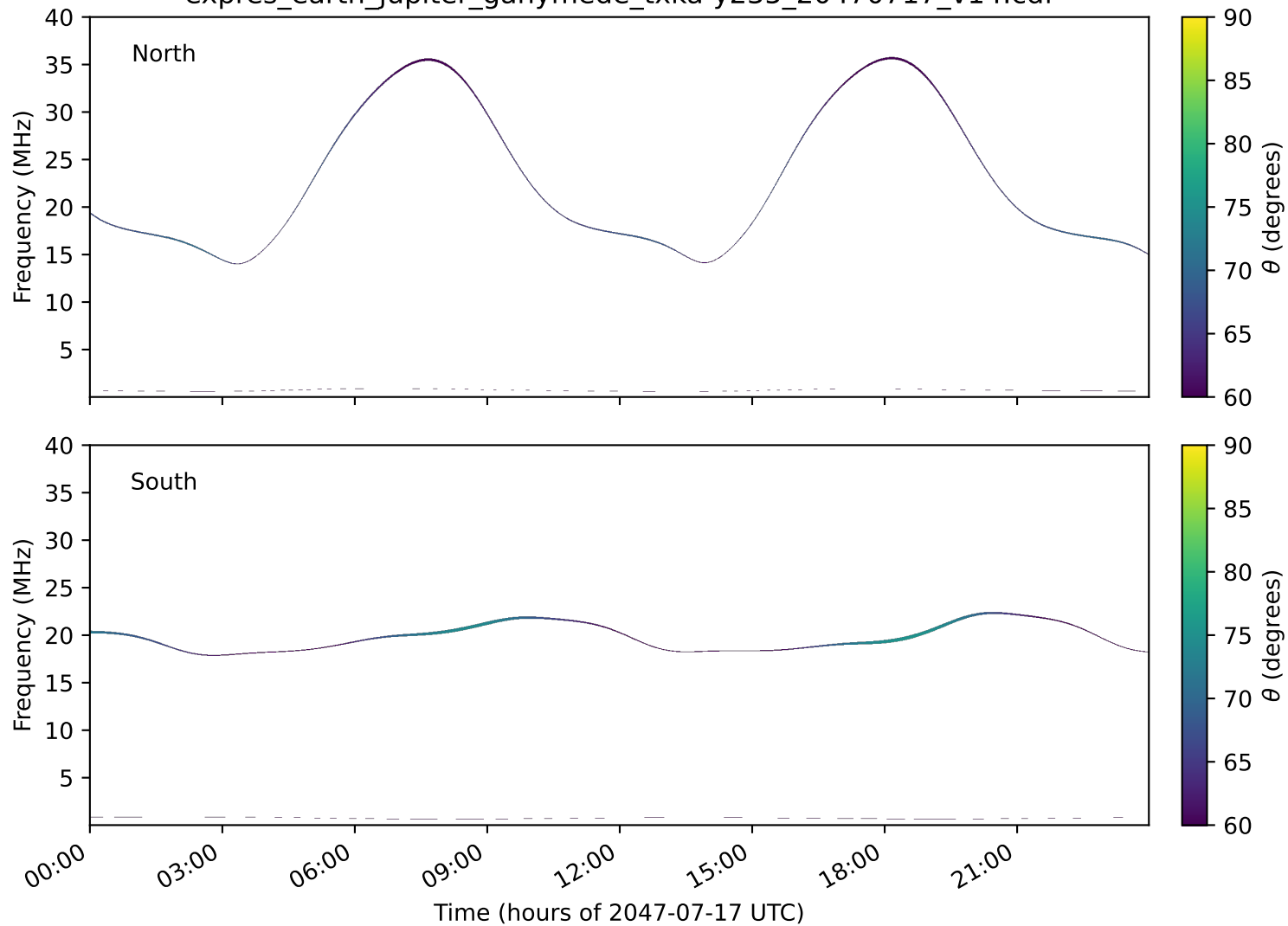
expres_earth_jupiter_ganymede_txka-y235_20470717_v14.cdf
