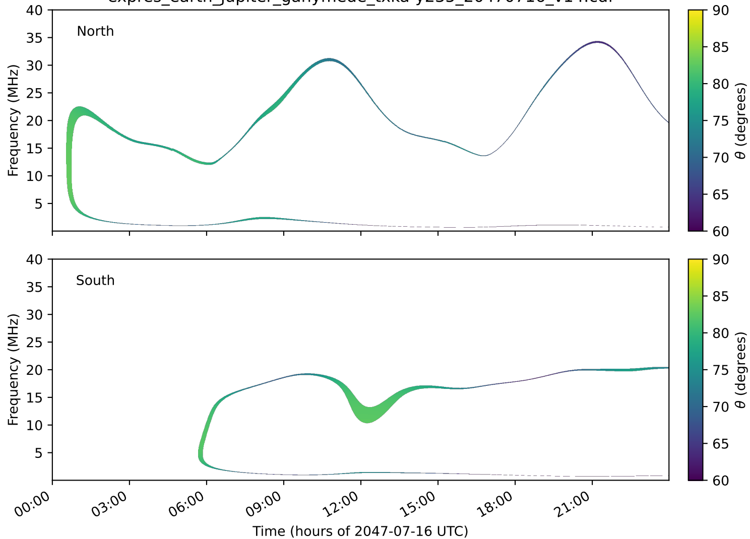
expres_earth_jupiter_ganymede_txka-y235_20470716_v14.cdf
