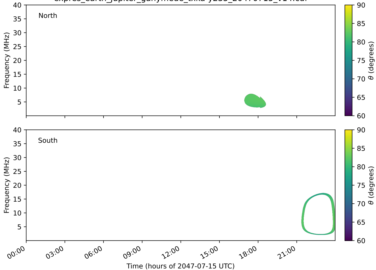
expres_earth_jupiter_ganymede_txka-y235_20470715_v14.cdf
