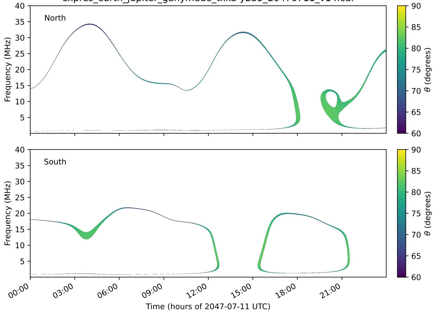
expres_earth_jupiter_ganymede_txka-y235_20470711_v14.cdf
