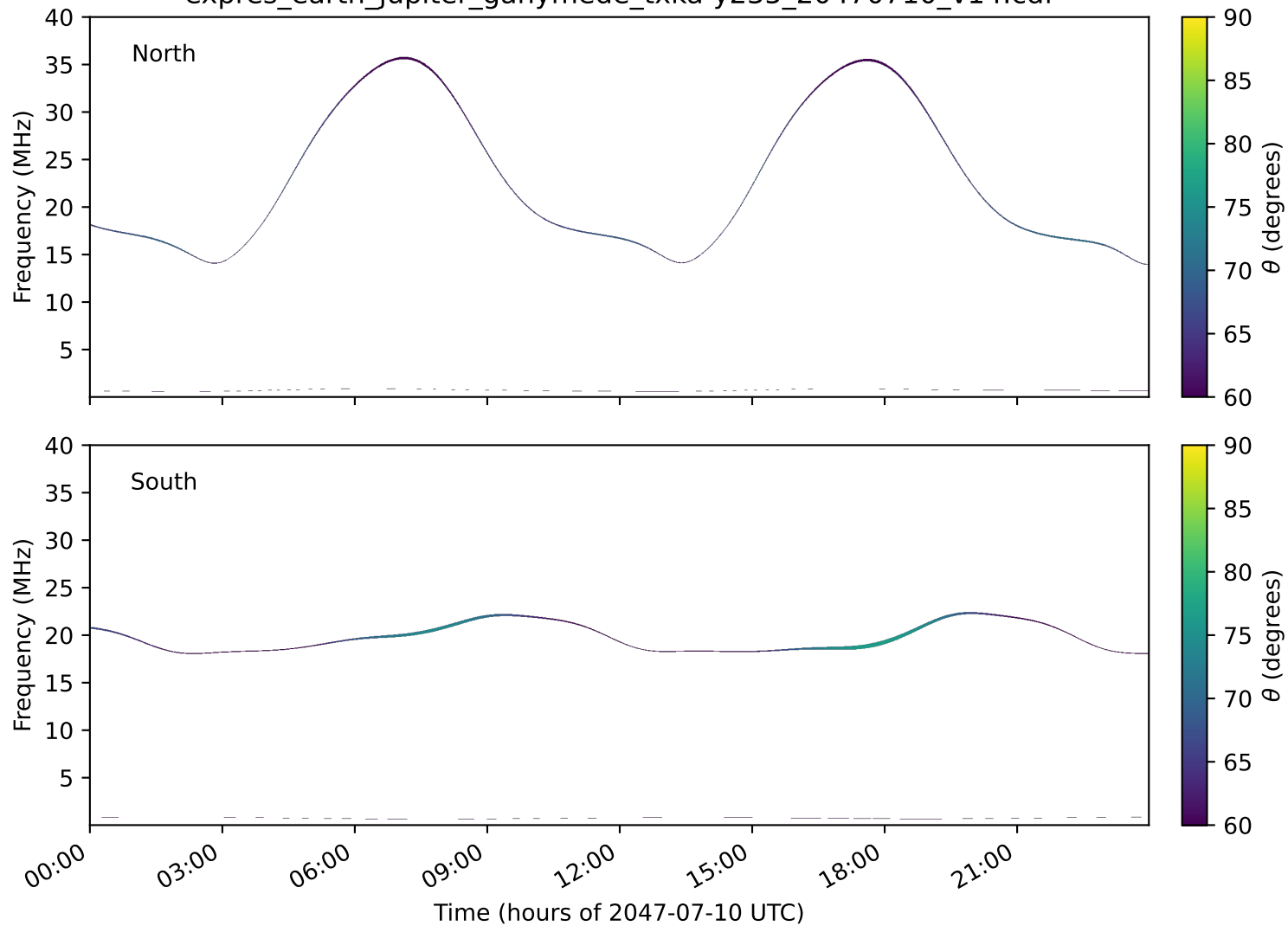
expres_earth_jupiter_ganymede_txka-y235_20470710_v14.cdf
